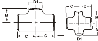
UNEQUAL TEE & CROSS
