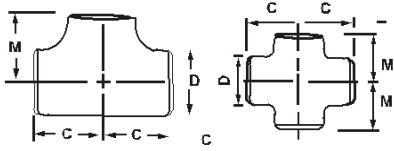
EQUAL TEE & CROSS
